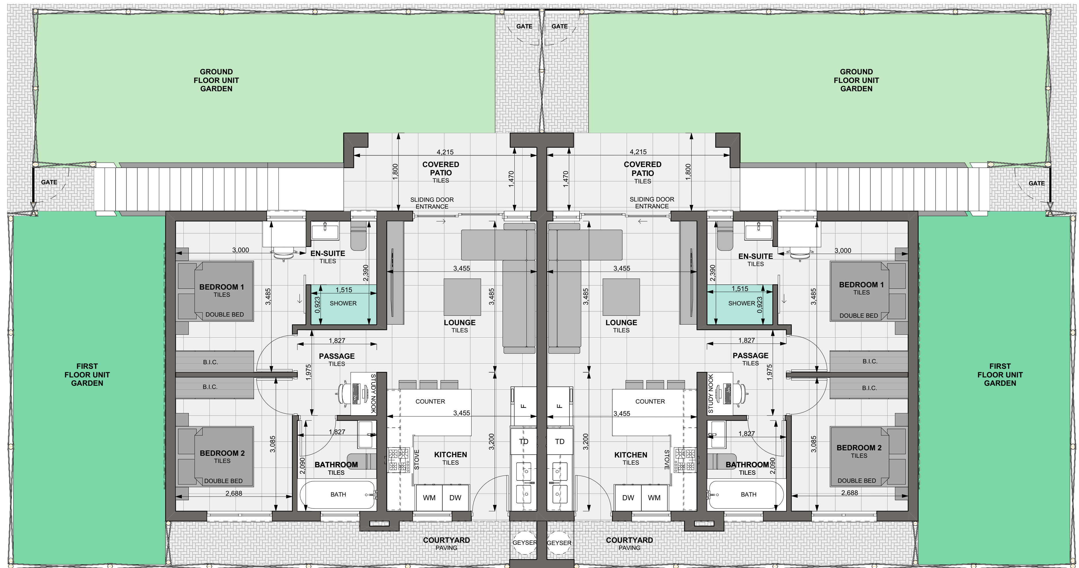
GROUND FLOOR SCALE 1:50
